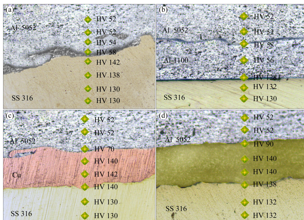
Fig. 14 Vickers microhardness variation across various interlayered explosive clads: (a) No interlayer; (b) Al 1100; (c) Pure copper; (d) SS 304
