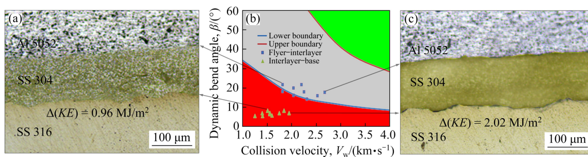
Fig. 10 Effect of SS 304 interlayer on microstructures (a, c) and biaxial welding window (b) of Al 5052–SS 316 explosive clad
